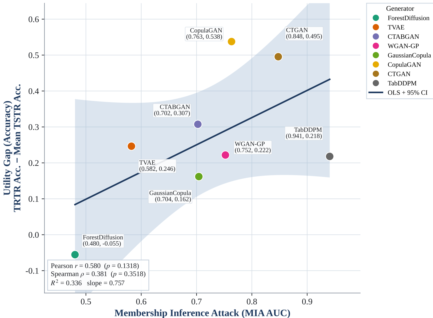
Forest Cover: MIA vs Utility Gap (Accuracy)
